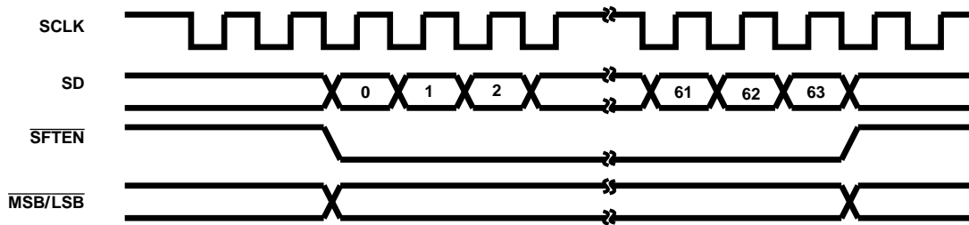
FIGURE 2A. FREQUENCY LOADING ENABLED BY \overline{\text{SFTEN}}
