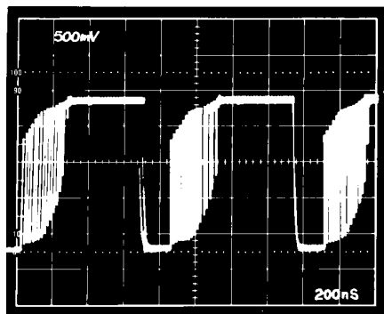
Photograph 1. AD9901 Output Waveform ( F_0 \ll F_1 )
