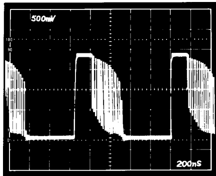
Photograph 2. AD9901 Output Waveform ( F_0 \gg F_1 )
