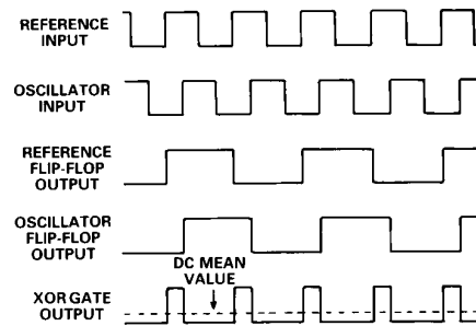
Figure 4. Timing Waveforms ( \phi_{OUT} Lags \phi_{IN} )
