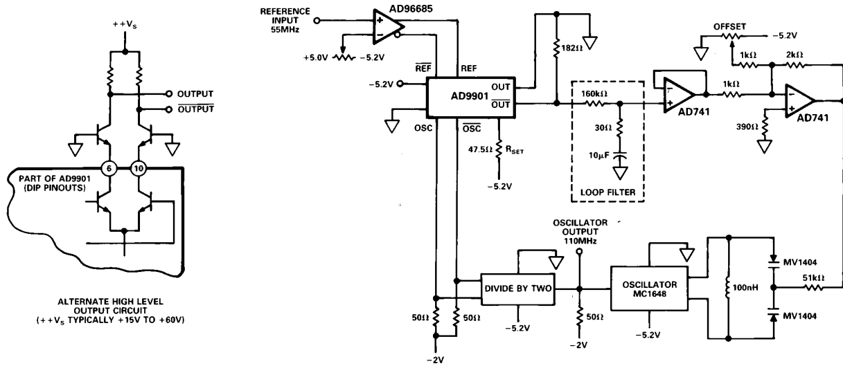
Phased-Locked Loop Using AD9901
