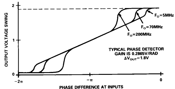
Figure 5. Phase Gain Plot
