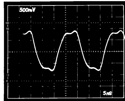
Photograph 3. AD9901 Output Waveform ( F_0 = F_1 = 50 \text{ MHz} )
